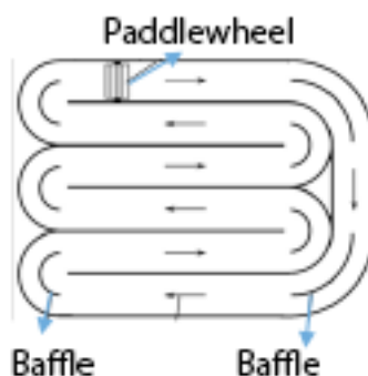
Figure 1: A simplified diagram of a raceway pond.
