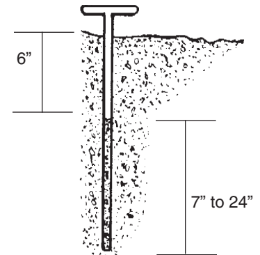
Figure 3. A soil probe is a good tool for obtaining soil samples. Push the tube to the six-inch depth and remove the core. Then take the seven to 24-inch core through the same hole for the subsoil test.
