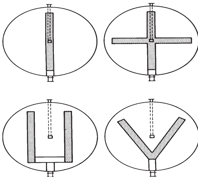
Figure 5. Common patterns for aeration ducts.
