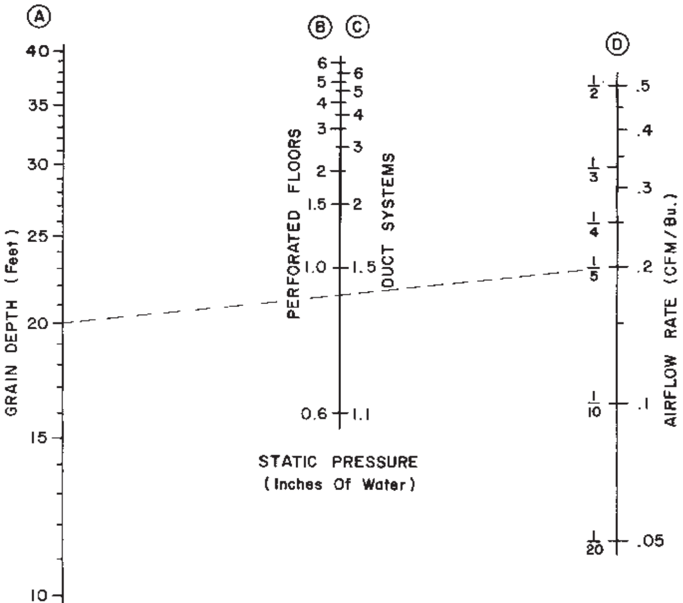
Nomograph 2. Expected static pressure for corn or soybeans.
