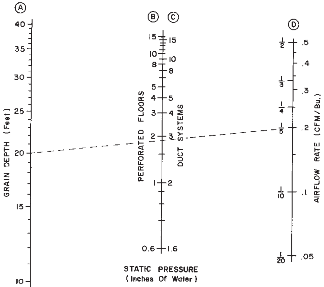
Nomograph 3. Expected static pressure for wheat, grain sorghum, oats, barley, or rye.
