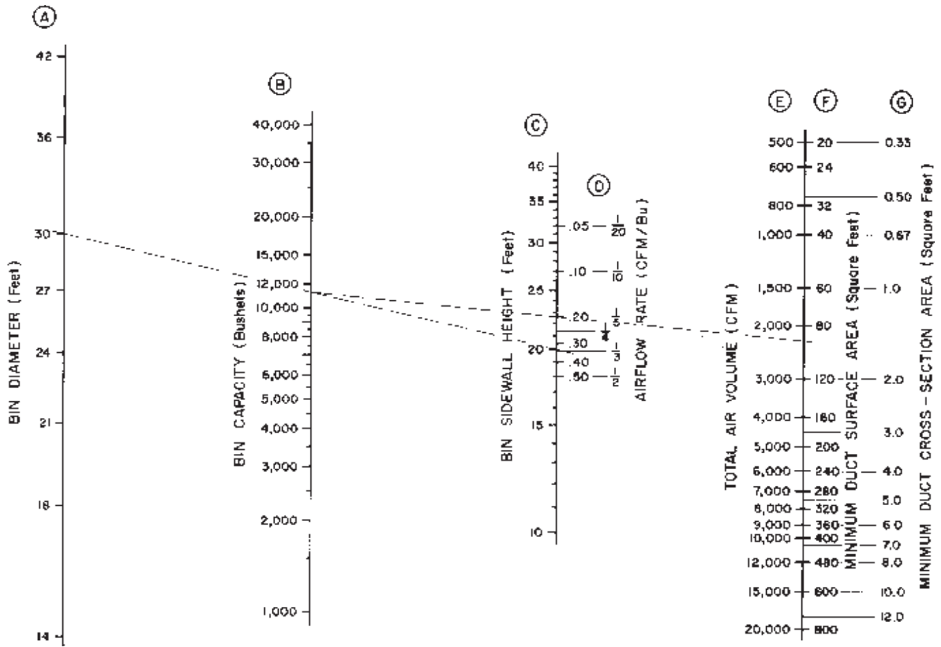
Nomograph 1. Bin capacity, total air volume and minimum duct areas.
