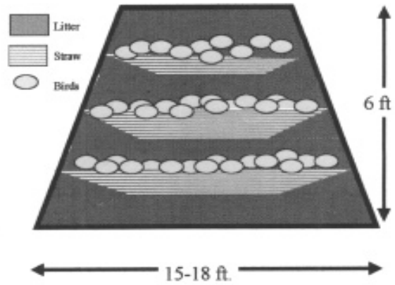
Figure 2. Cross-section of a large-scale, outside mortality composting system showing ingredients, relative proportions, and dimensions.
